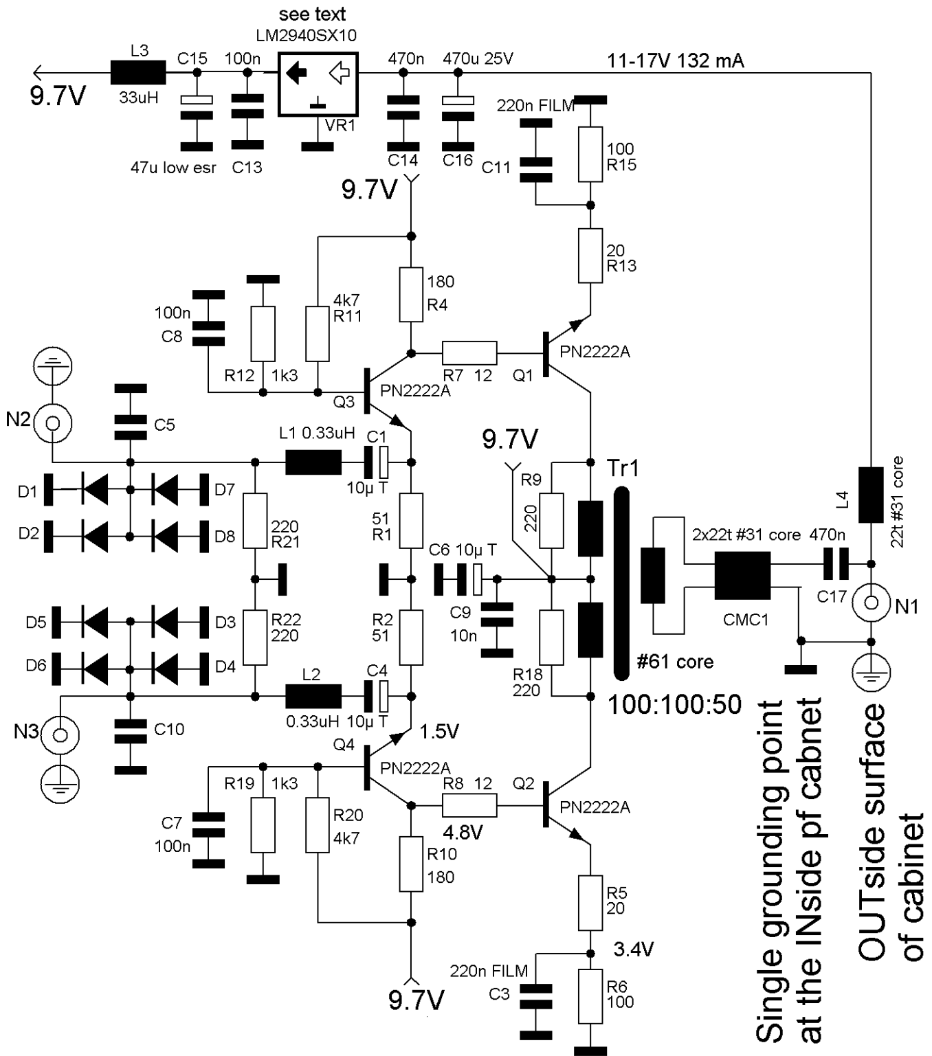
pa0nhc / LZ1AQ RXloop amplifier - Copyright 20200104
