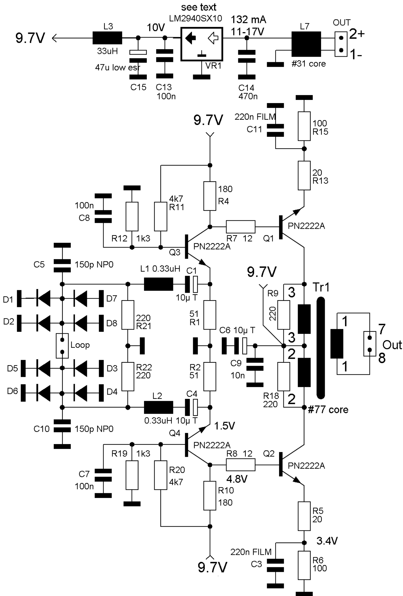
pa0nhc / LZ1AQ RXloop amplifier - pa0nhc 20190828-p96
