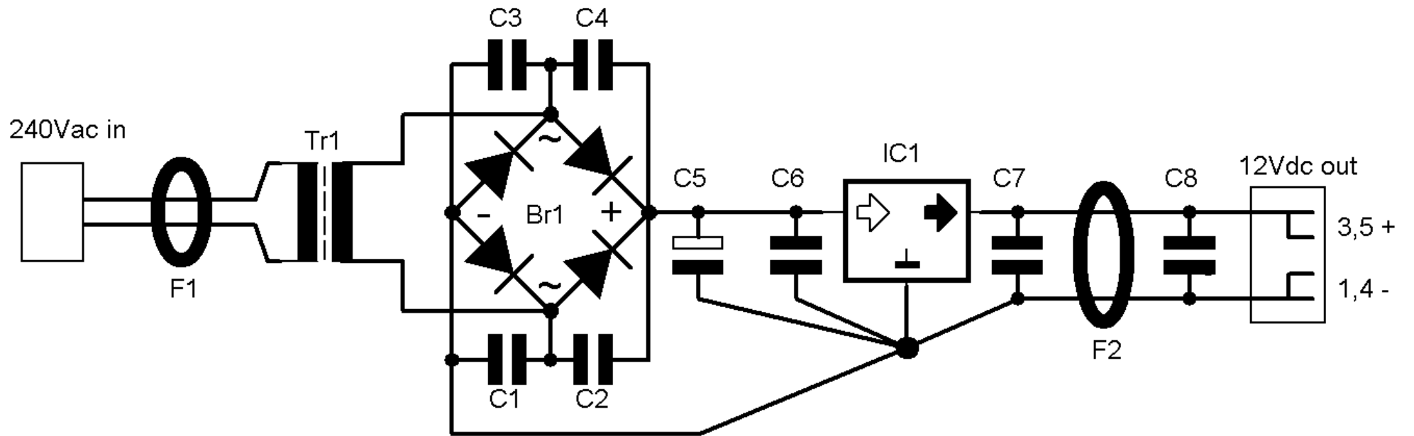
Pa0nhc noiseless 12V/135mA power supply
