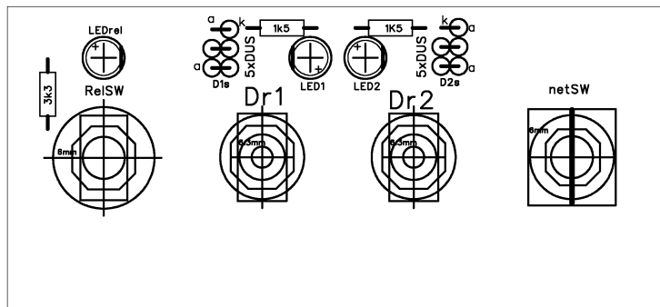
pe0rig/pa0nhc drill plan FRONT
