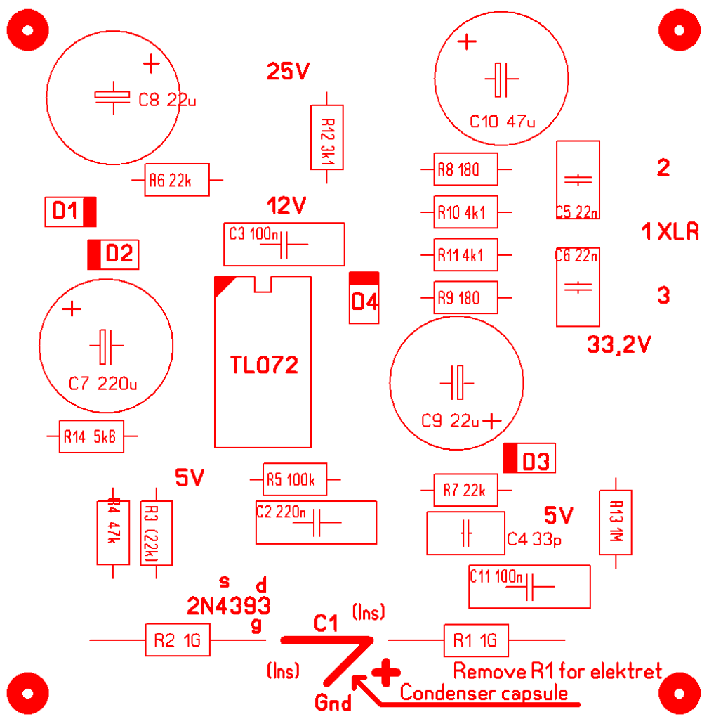
CmicInterface SILK pa0nhc 20080110
