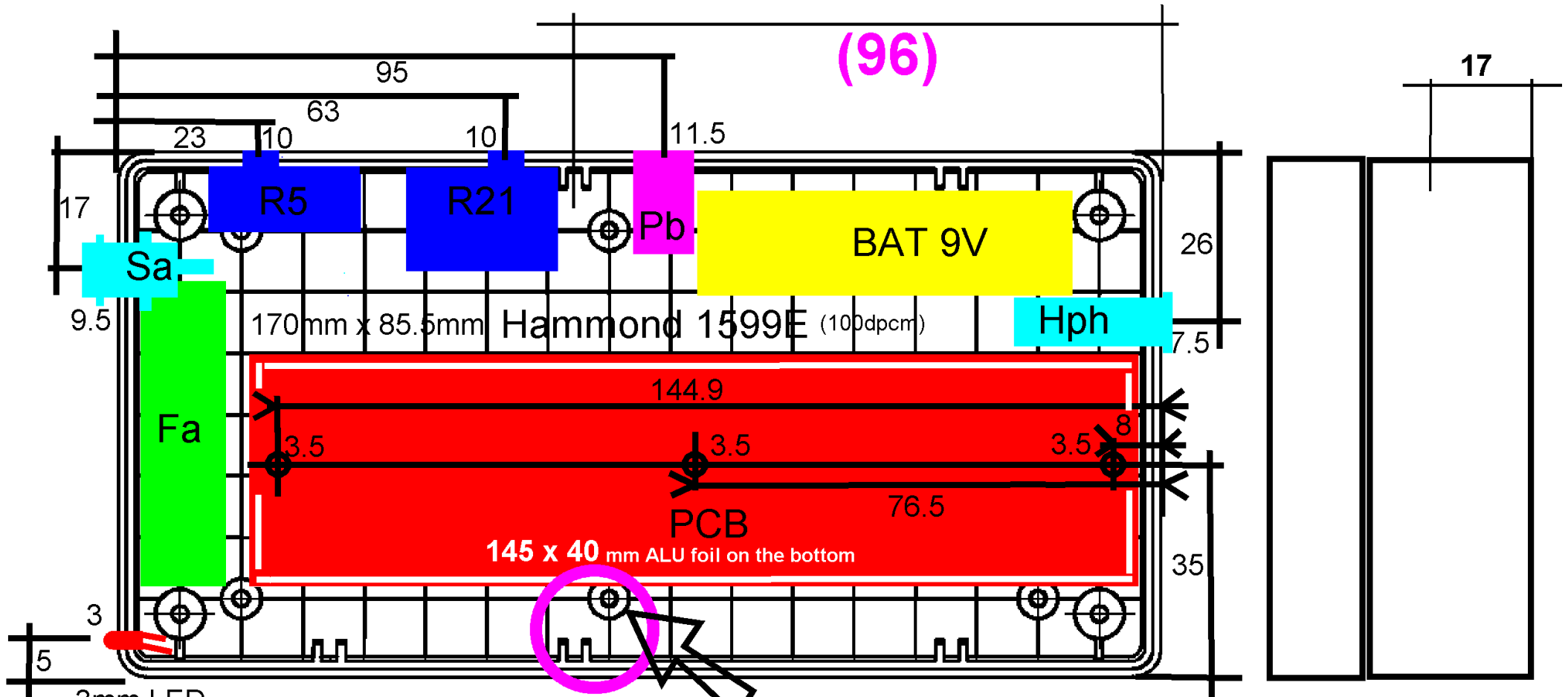
Drill plan ARDFrx80-7 ver. 20171014
