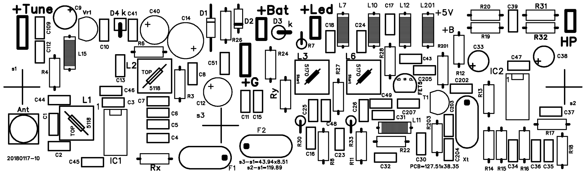
ARDFrx2-2 PCB 20180117-10
