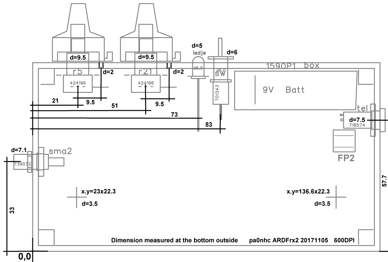
ARDFrx2 housing 20171217
